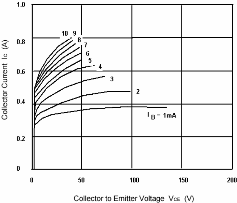
Fig.4 Static Characteristic
